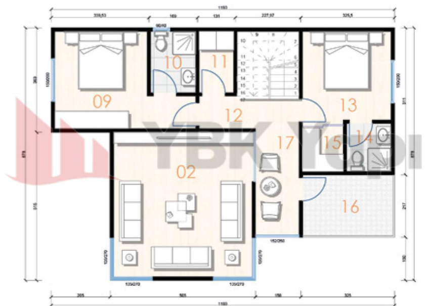
BİRİNCİ KAT PLANI 87,0 m 2
