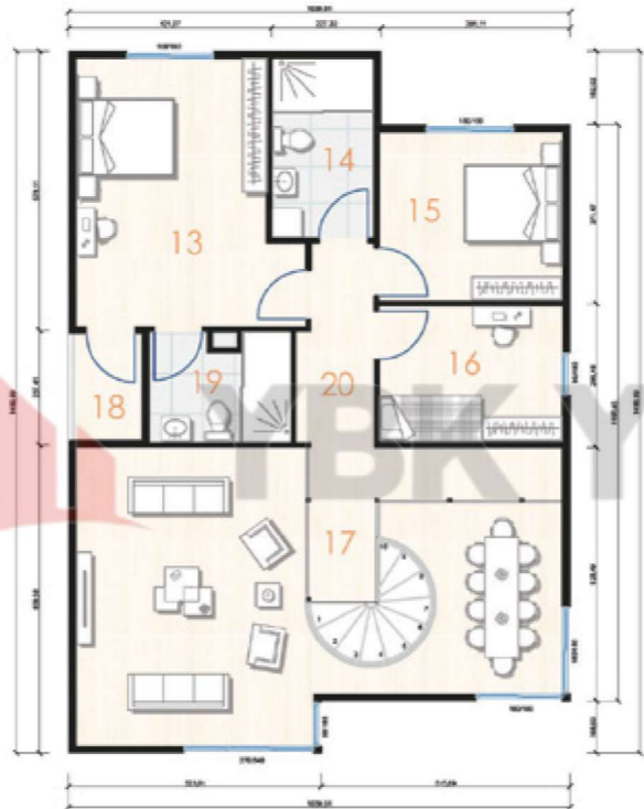
BİRİNCİ KAT PLANI 140,0 m 2
