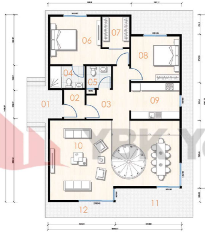
ZEMİN KAT PLANI 137,0 m 2
