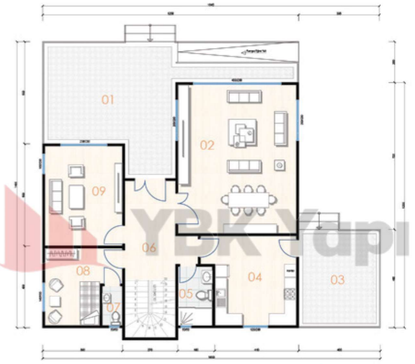
ZEMİN KAT PLANI 128,0 m2
